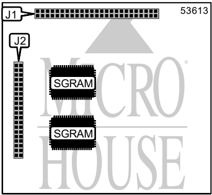
2MB Upgrade Board
