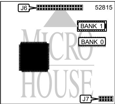
MPEG Upgrade Card
