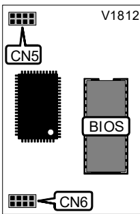
TELETEXT DAUGHTER BOARD
